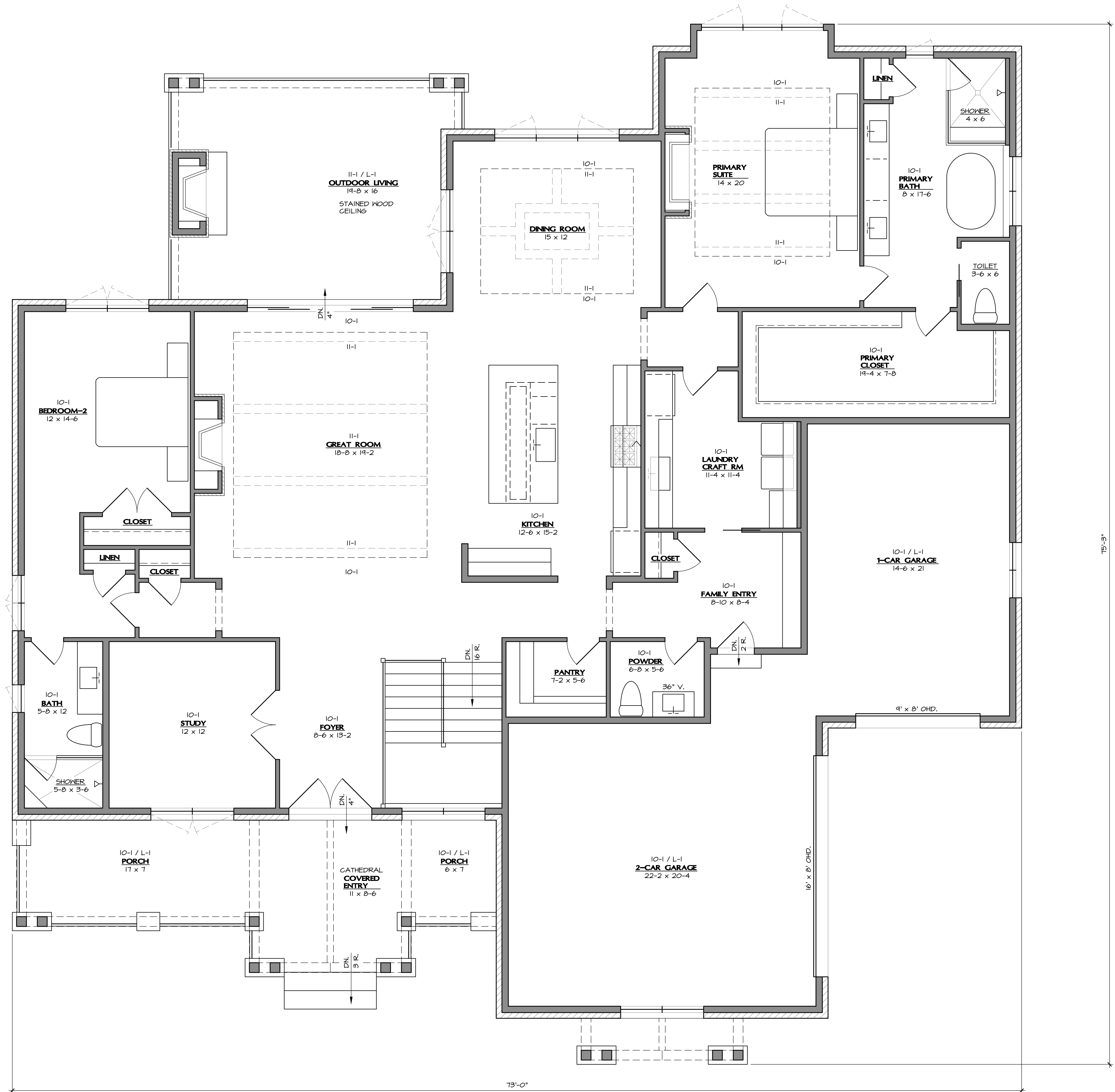
MAIN LEVEL INTERIOR DESIGN PLAN 1/4" = 1'-0" LIVING AREA: 2813 SF 3-CAR GARAGE: 891 SF COVERED ENTRY: 306 SF OUTDOOR LIVING: 322 SF TOTAL UNDER ROOF: 4322 SF
